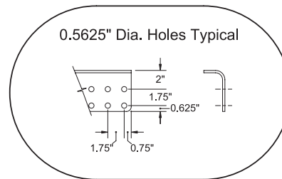
Bus Detail
